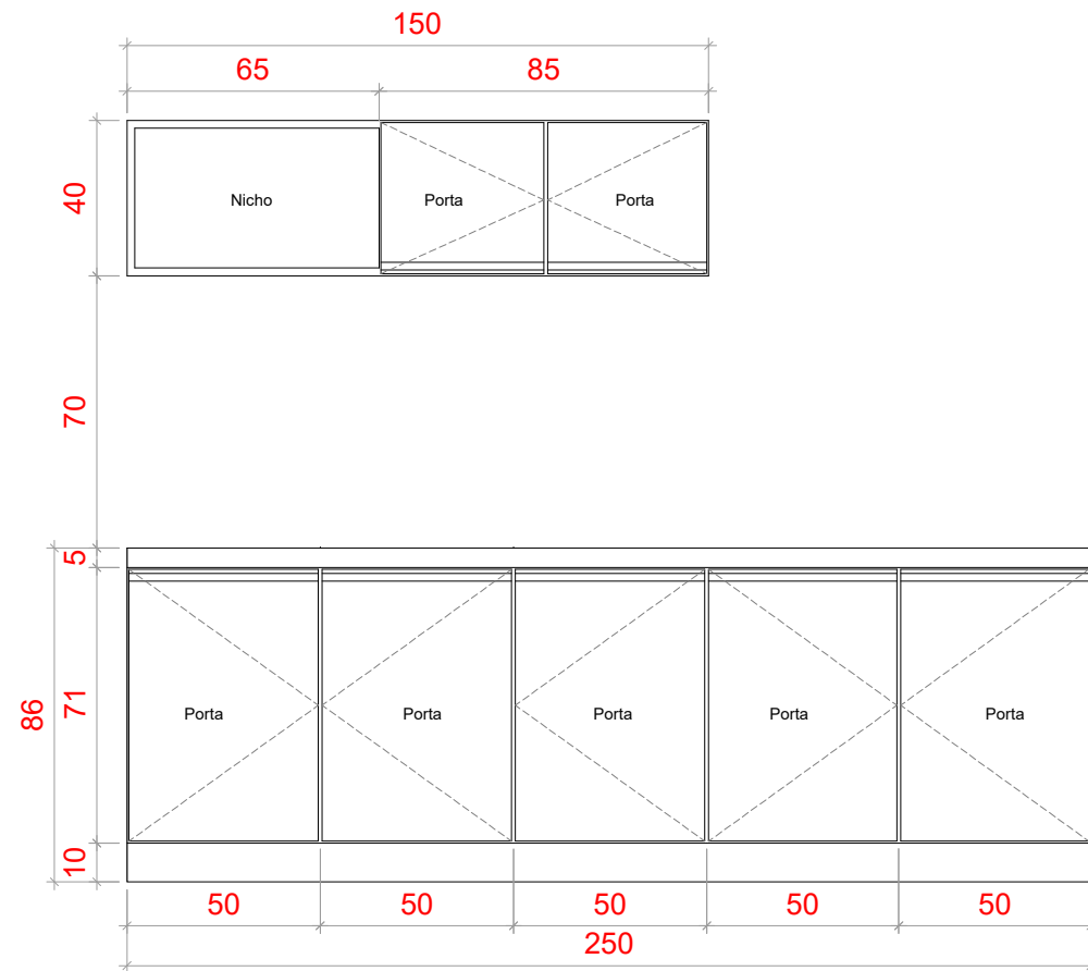
Vista Frontal
