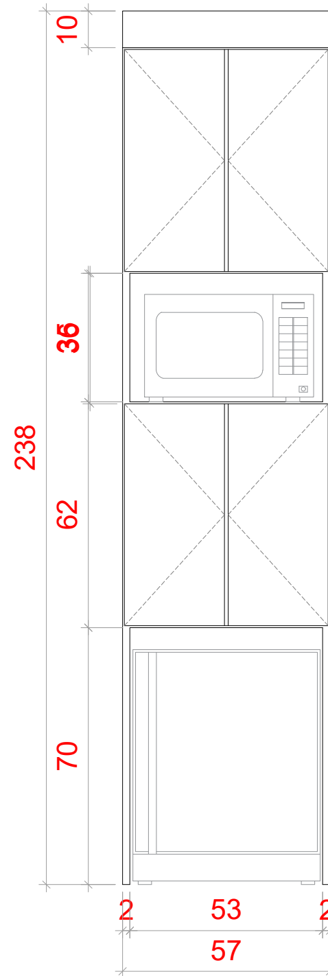
Vista Frontal
