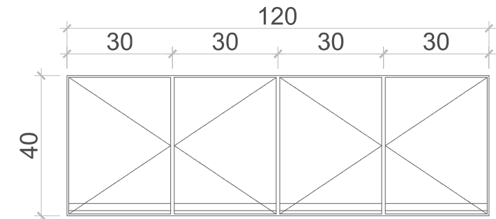
Vista Frontal
