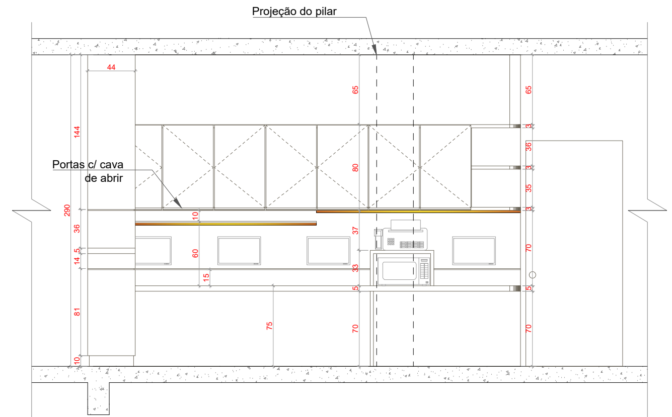
Vista Frontal
