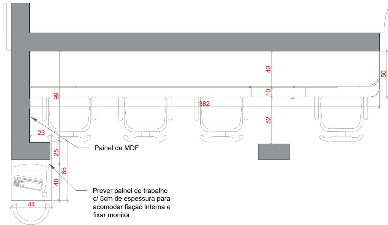
Vista Frontal
